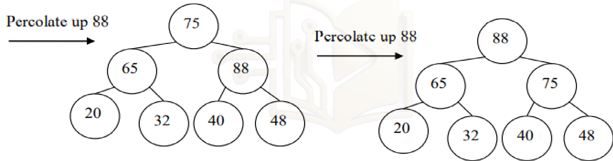
Fig: Creating Max Heap
